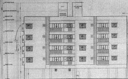
SOUTH SIDE ELEVATION (BLOCK-2)
