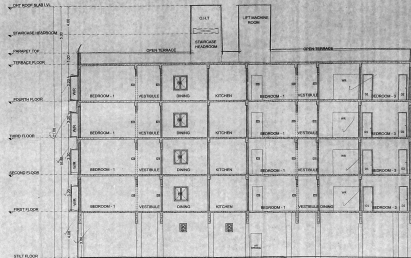
SECTION 'YY' (BLOCK-2)
